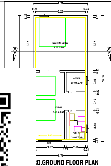
G.O.GROUND FLOOR PLAN
