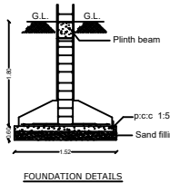
FOUNDATION DETAILS
