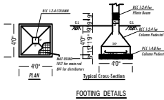
FOOTING DETAILS
