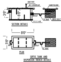
SEPTIC TANK AND DISPERSION TRENCH DETAILS
