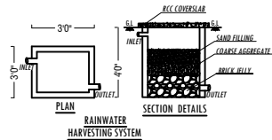
RAINWATER HARVESTING SYSTEM
