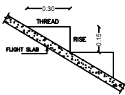
STAIRCASE DETAILS (NOT TO SCALE)
