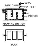
SEPTICTANK DETAILS NOT TO SCALE
