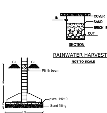
FOUNDATION DETAILS
