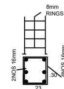
COLUMN DETAILS
