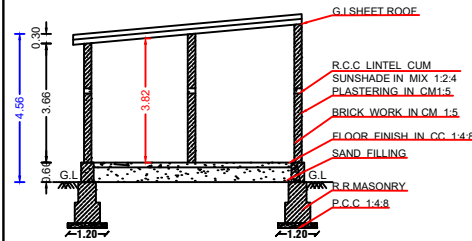
SECTION ON-'AB'
