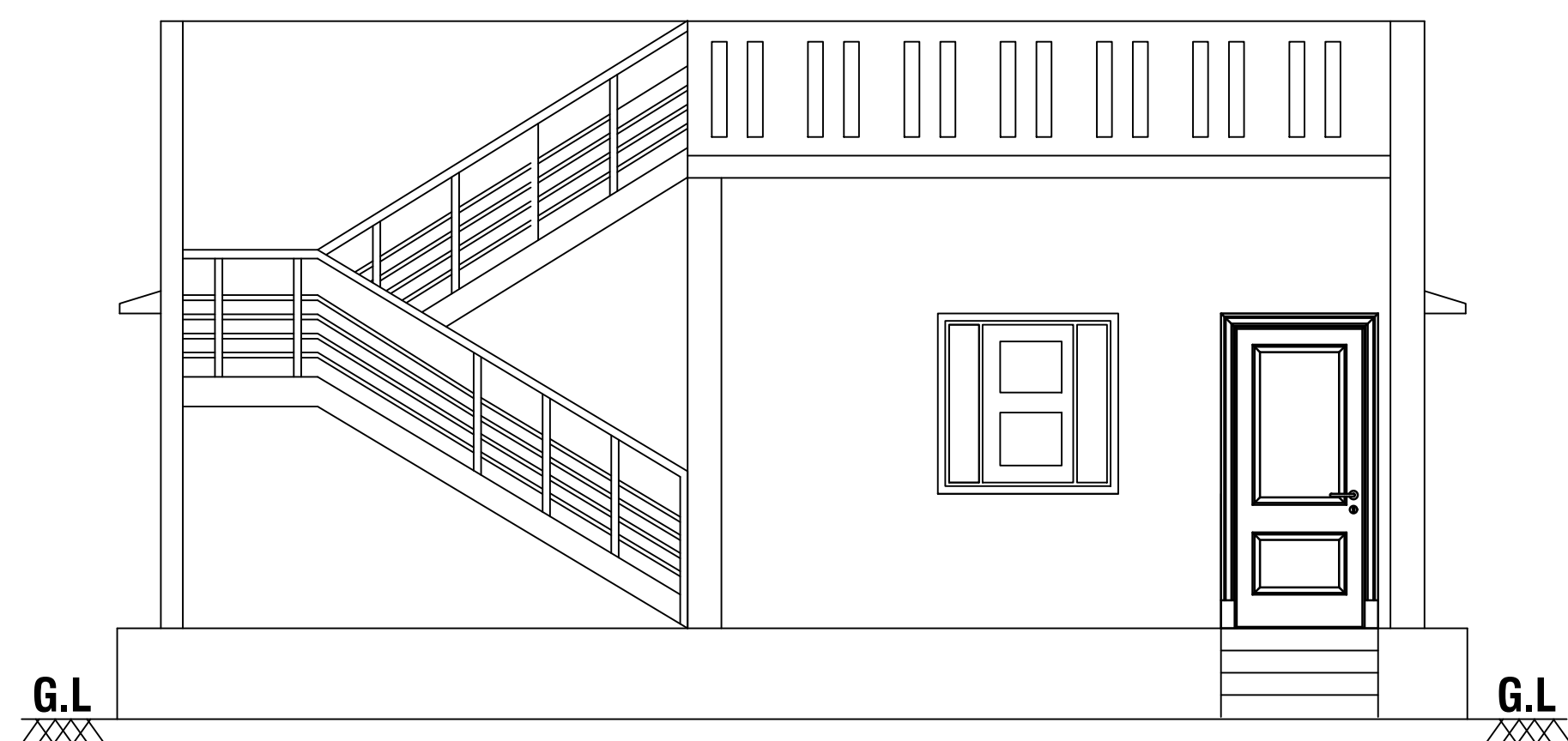
Overall Dimensions: Total Width: 8.54 Total Depth: 11.12 Room Details: BED ROOM: 3.35 X 3.05 (Two rooms) HALL: 4.74 X 5.65 DINNING: 3.35 X 3.05 KITCHEN: 3.35 X 2.45 TOILET: 1.54 X 1.83 POOJA: 1.54 X 1.07 PORTICO: 4.98 X 2.44 Other Features: - Staircase: Located in the Portico area. - Doors: D, D1, MD. - Windows: W, W1. - Vents: V. - Total Area: 1150 sq. ft.
