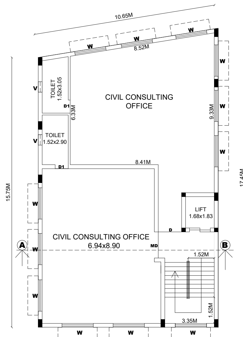
TYPICAL FLOOR PLAN (FIRST & SECOND FLOOR)
