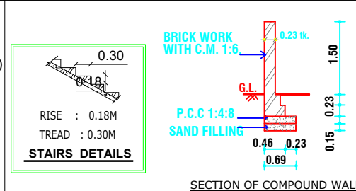
SECTION OF COMPOUND WALL
