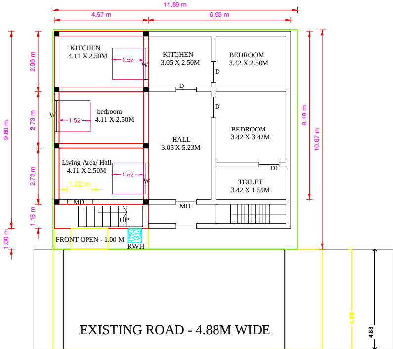
PROP .GROUND FLOOR PLAN EXISTING GROUND FLOOR PLAN
