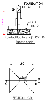
SECTION - 'CD'
