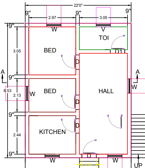
G.F. PLAN
