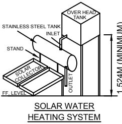
SOLAR WATER HEATING SYSTEM
