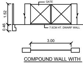
COMPOUND WALL WITH DWARF WALL DETAILS
