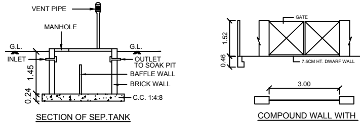
SECTION OF SEP.TANK
