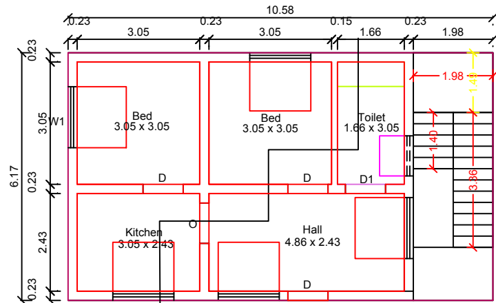
PRO.GROUND FLOOR PLAN
