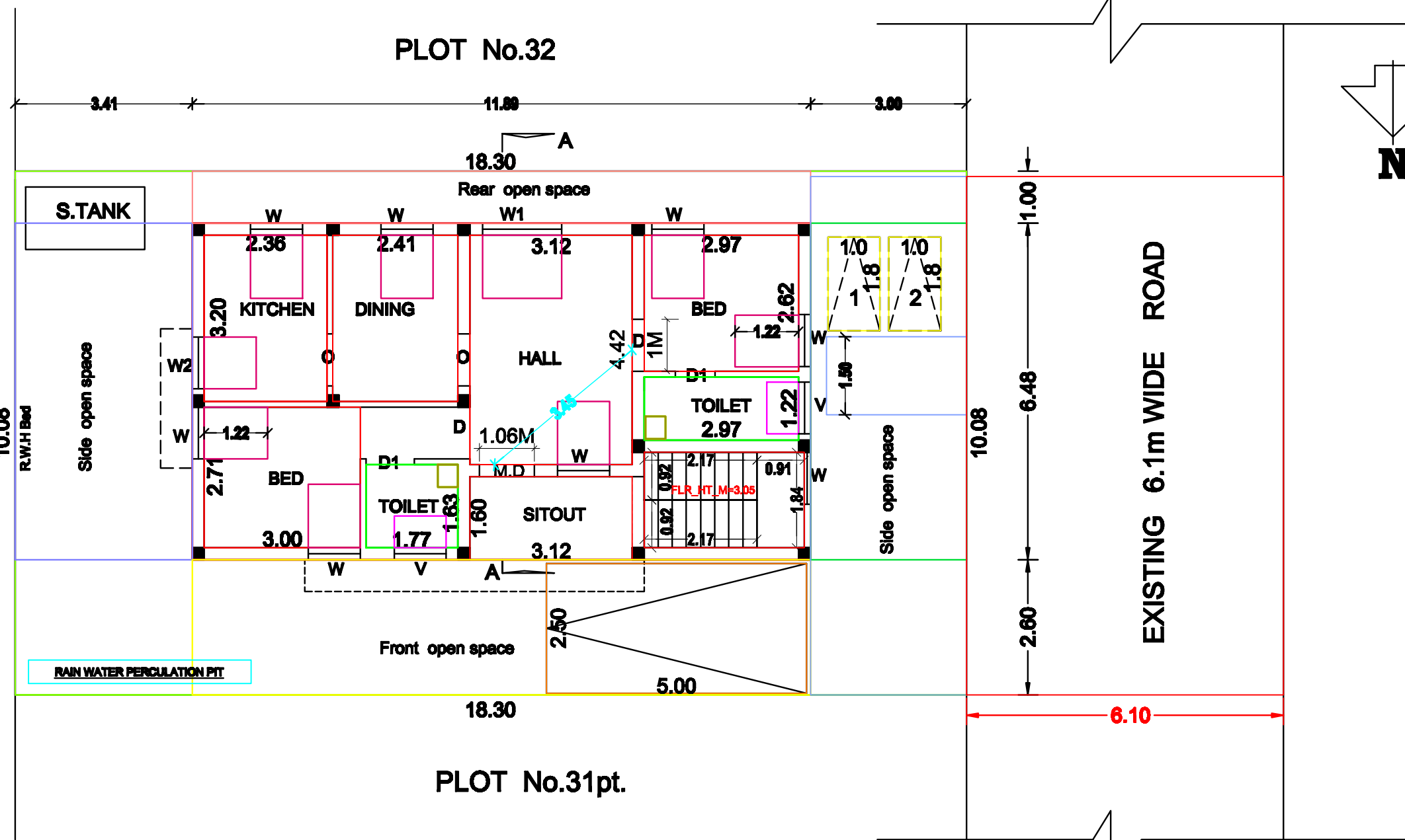
SITE CUM EXISTING GROUND FLOOR PLAN
