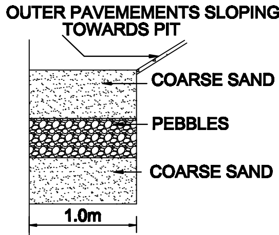
RAIN WATER PERCOLATION BED
