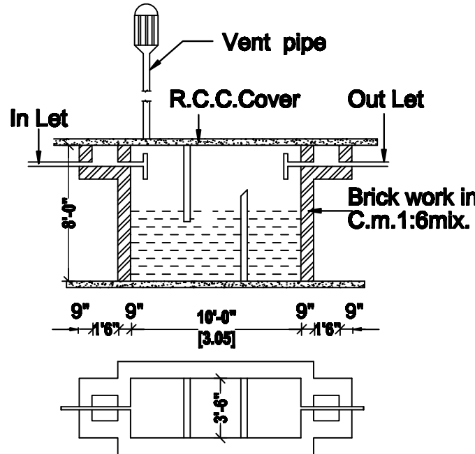
SEPTIC TANK DETAILS (NOT TO SCALE)
