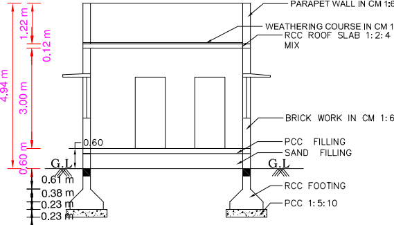
SECTION ON KA
