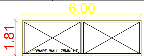
MAIN GATE
