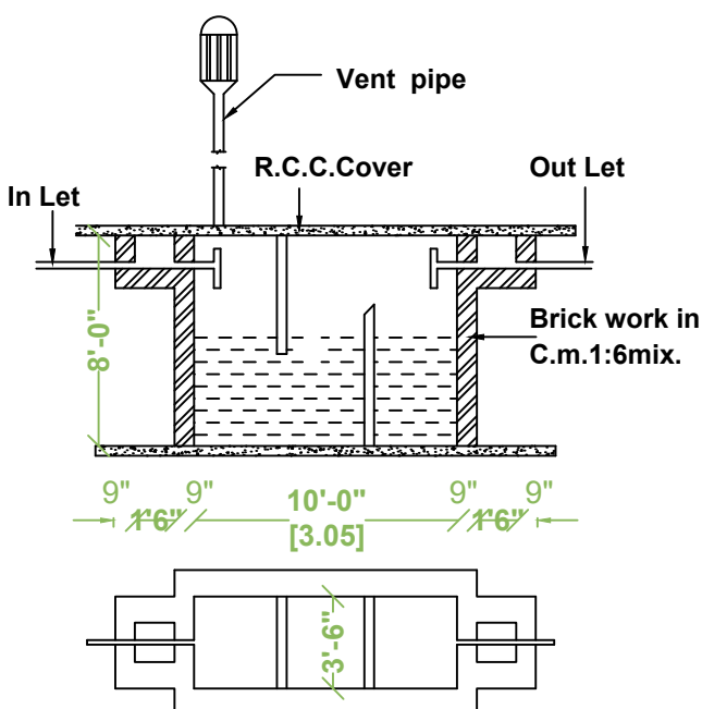
SEPTIC TANK DETAILS (NOT TO SCALE)
