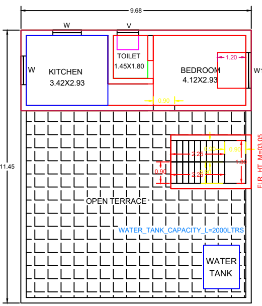
PROPOSED TERRACE PLAN
