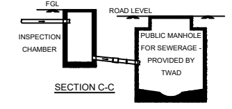
WASTE DISPOSAL DETAIL
