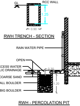
RWHT TRENCH - SECTION
