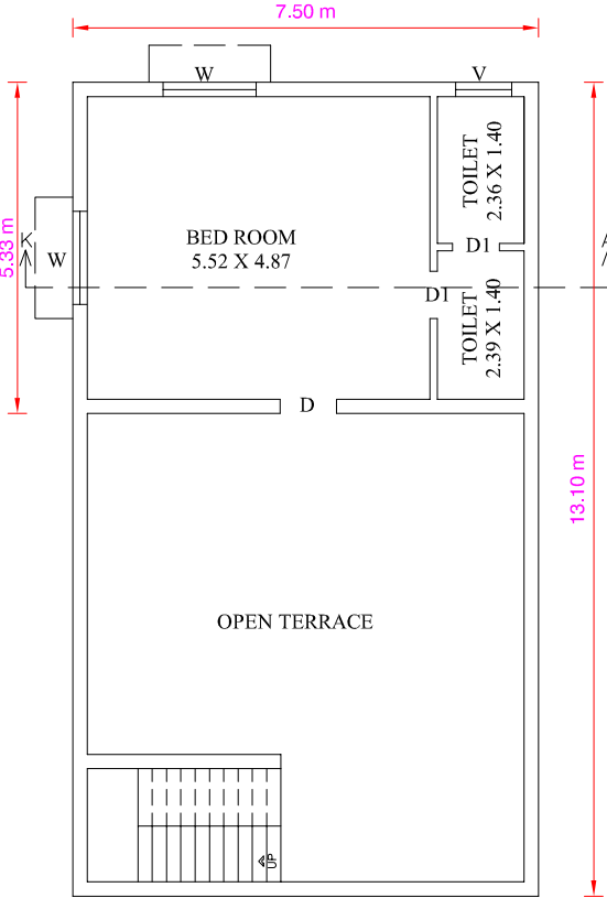
FIRST & TERRACE FLOOR PLAN
