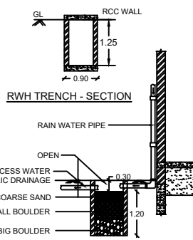
RW-H - PERCOLATION PIT
