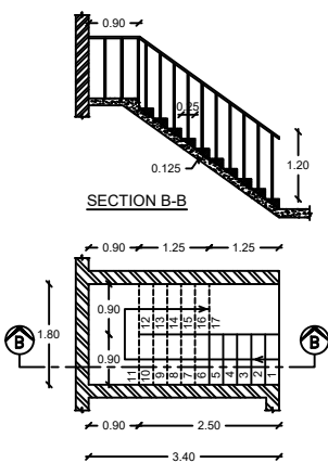
STAIRCASE PLAN
