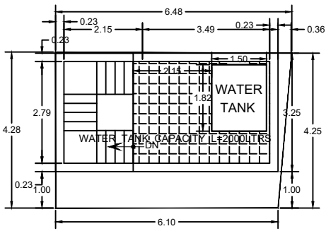
PROPOSED TERRACE PLAN
