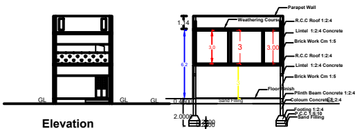
Section Section - AA
