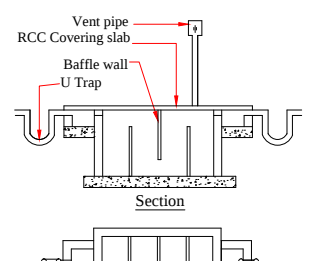
Septic Tank With U Trap Not To Scale
