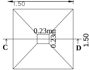
SECTION - 'CD'
