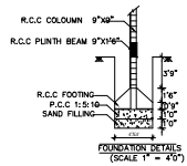
FOUNDATION DETAILS (SCALE 1"=4'0")
