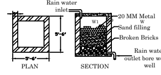
RAIN WATER HARVESTING TANK PLAN
