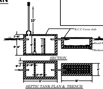
SEPTIC TANK PLAN & TRENCH
