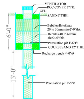
RAIN WATER STORAGE SCALE: 1"=4'-0"
