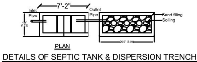
DETAILS OF SEPTIC TANK & DISPERSION TRENCH
