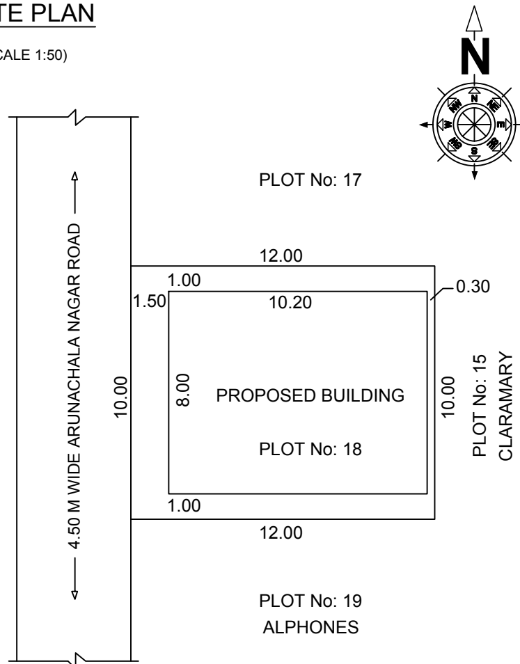
SITE PLAN
