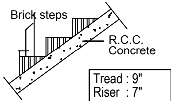
STAIRCASE DETAILS
