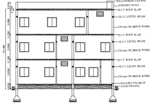
SECTION ON 'BK'
