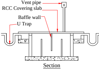
SECTION - 'CD'
