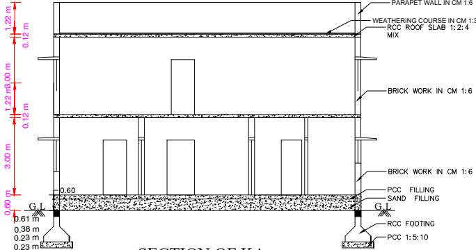
SECTION OF KA
