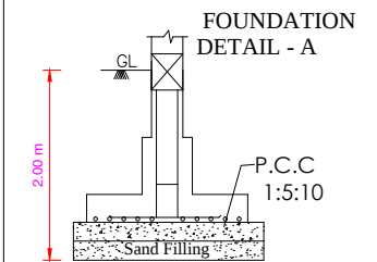
Isolated Footing -A (1.50X1.50) (Not to Scale)
