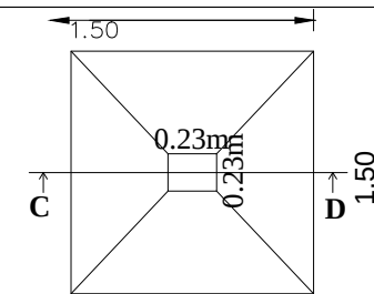
SECTION - 'CD'
