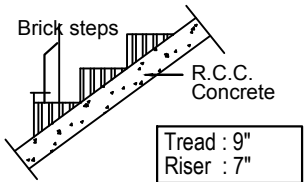
STAIRCASE DETAILS
