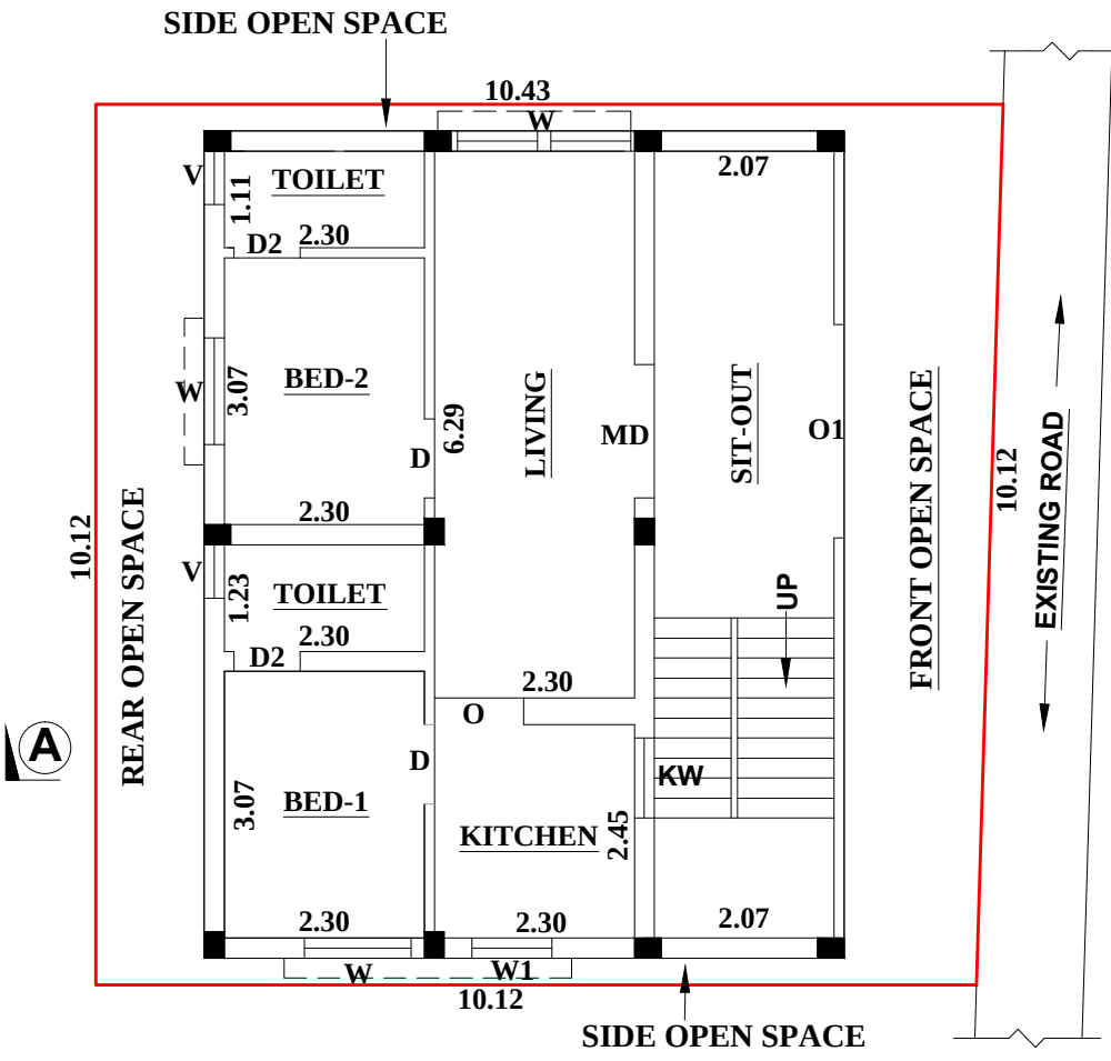
. SITE PLAN CUM GROUND FLOOR PLAN .
