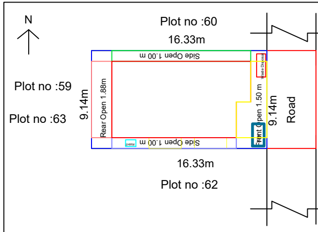
Site Plan
