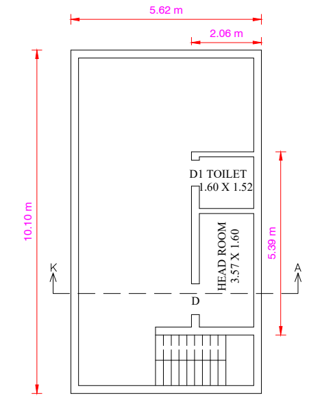
FIRST & TERRACE FLOOR PLAN
