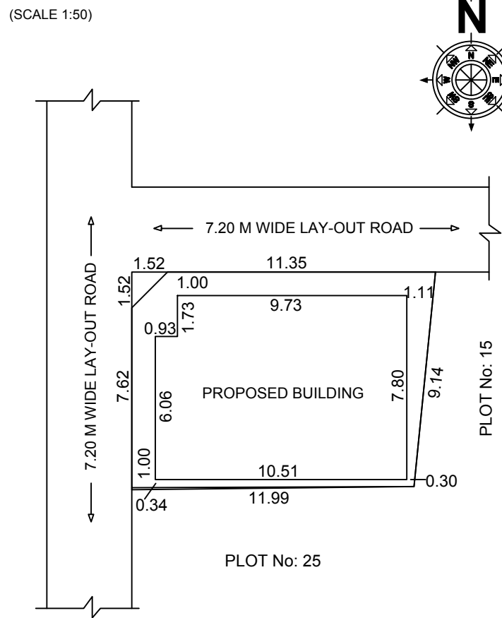
SITE PLAN
