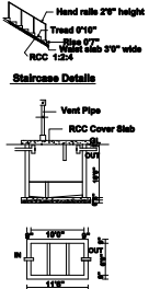
Septic Tank Details
