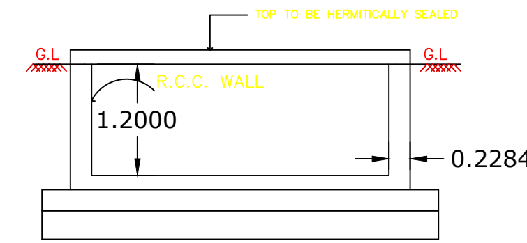
RWH_SECTION (SAMPLE) RWH_CAPACITY_L = 2000LTRS
