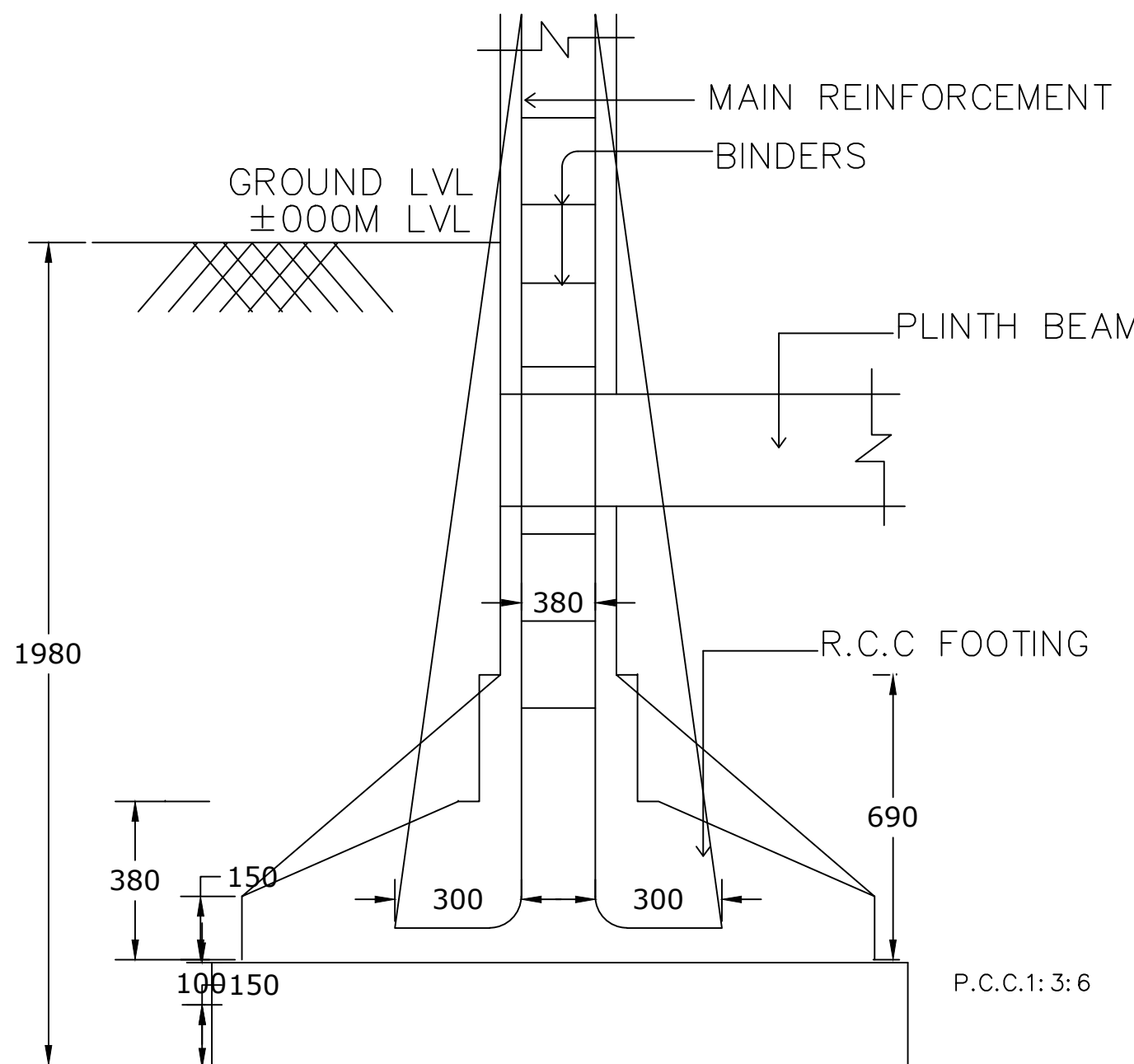
SECTION ON D-D
