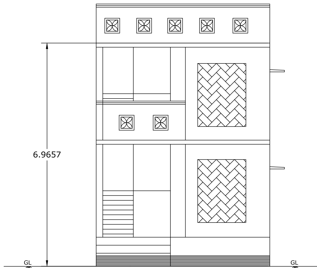
FRONT ELEVATION
