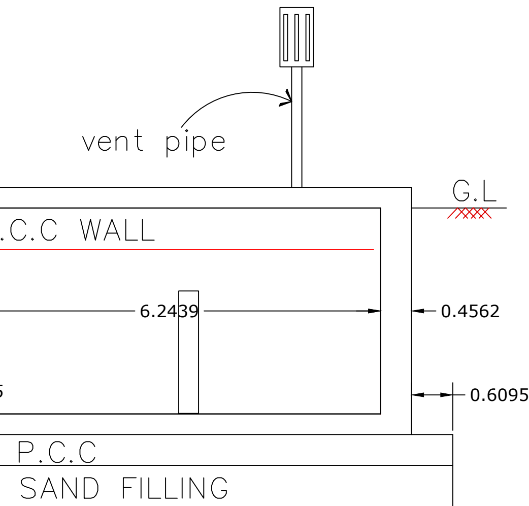
SECTION ON D-D
