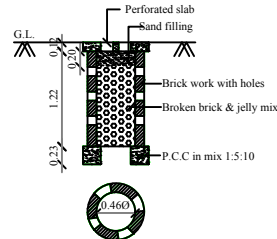
PERCOLATION PIT FOR 30 Sq. m. (Scale:- 1:50)
