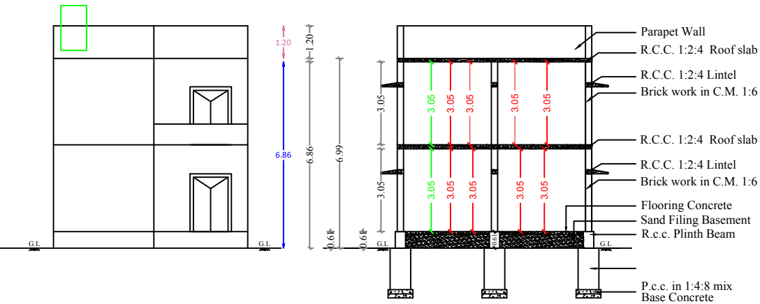
FRONT ELEVATION
