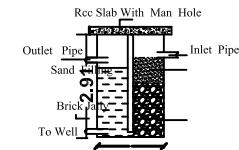
RWHTank Details
