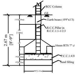
FOUNDATION DETAILS
