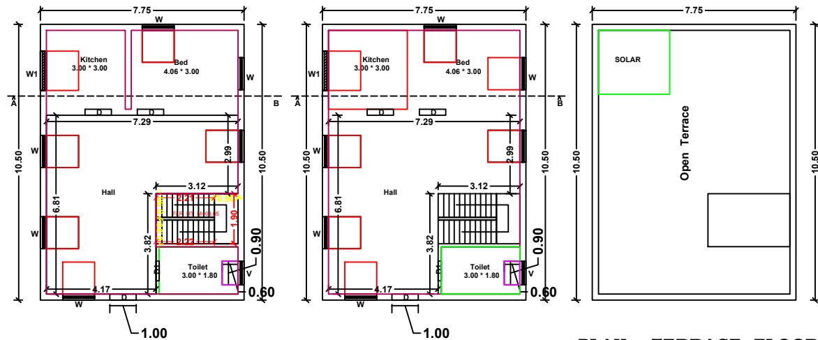
PLAN - GROUND FLOOR
