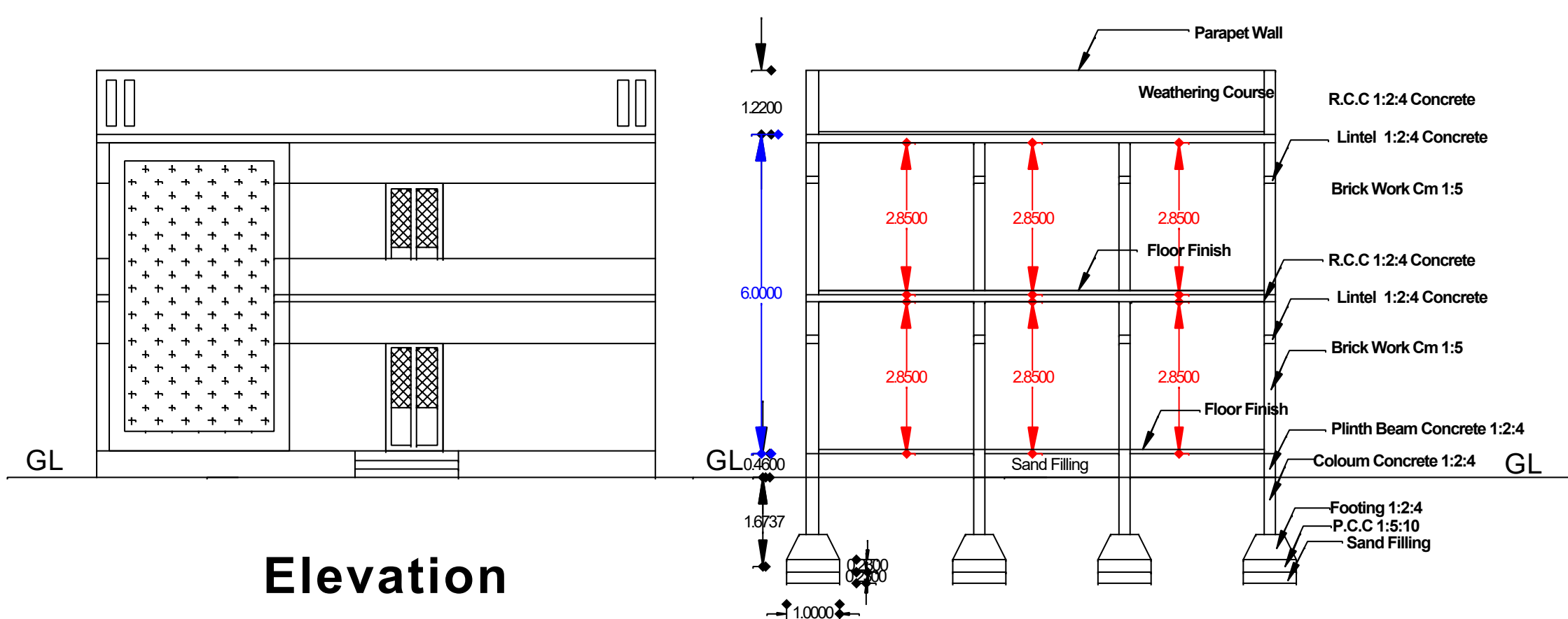
Section
