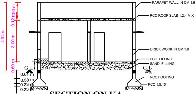
SECTION ON KA
