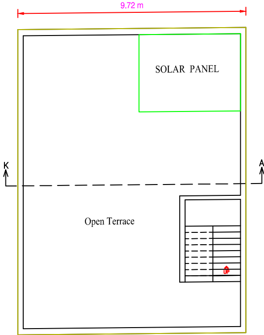
TERACE FLOOR PLAN
