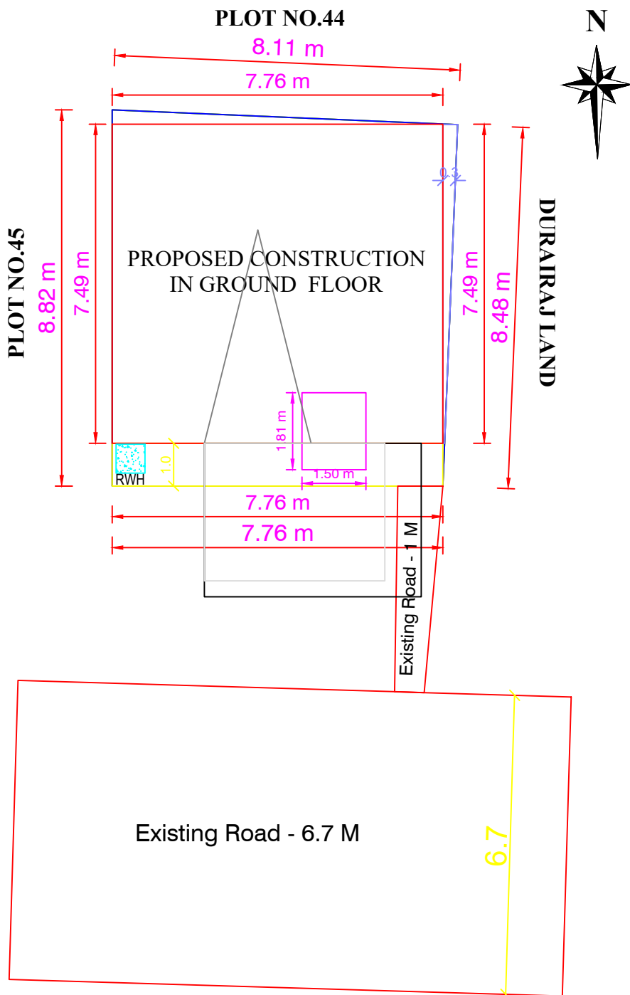
SITE PLAN
