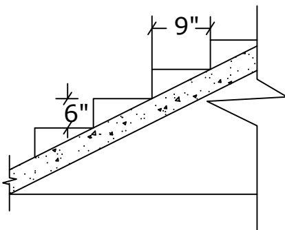
Staircase Detail Not To Scale
