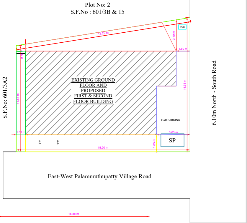
SITE PLAN
