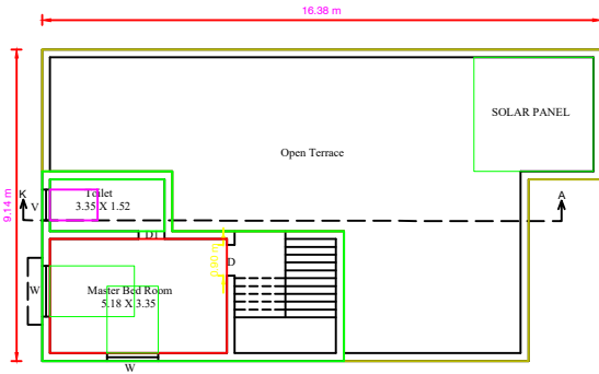
SECOND FLOOR & TERRACE FLOOR PLAN
