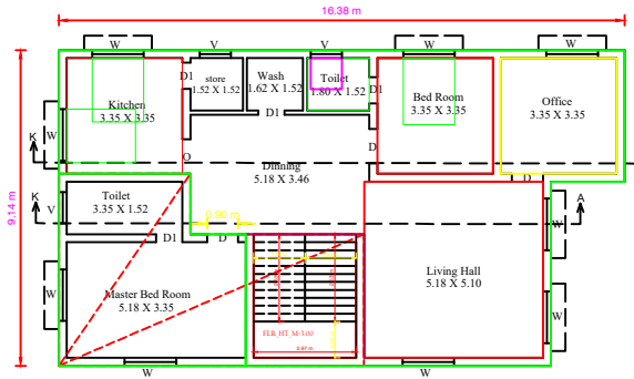
EXISTING & PROPOSED FIRST FLOOR PLAN
