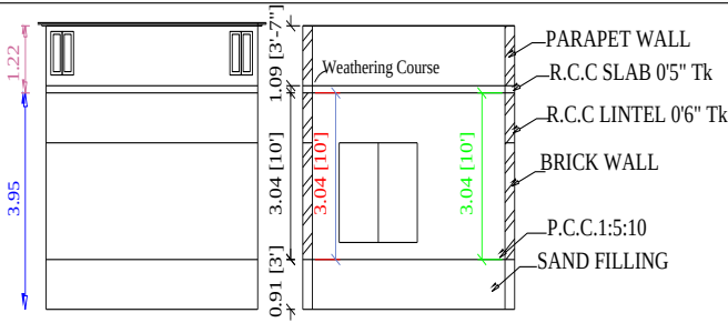
ELEVATION SECTION ON"AB"
