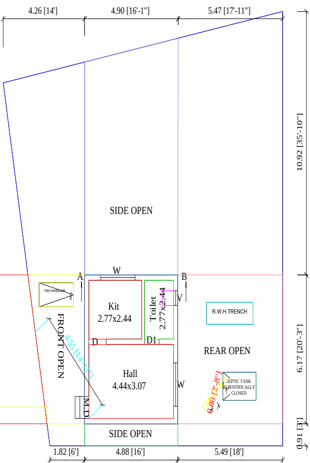
PRO.FIRST FLOOR (G+1 Residential)
