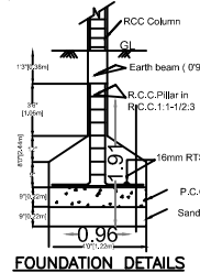
FOUNDATION DETAILS
