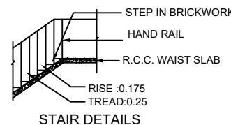
STAIR DETAILS
