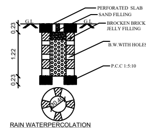
RAIN WATERPERCOLATION
