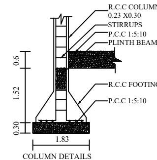
COLUMN DETAILS
