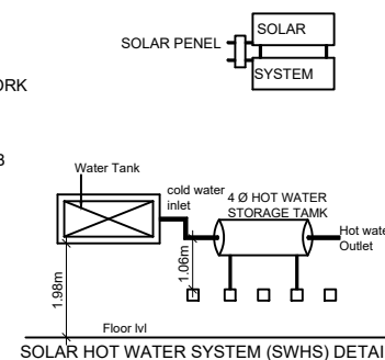
SOLAR HOT WATER SYSTEM (SWHS) DETAIL
