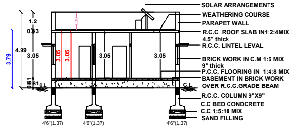
SECTION " AB "
