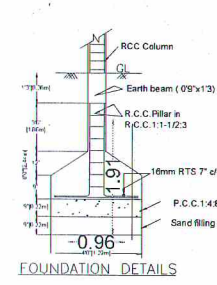
FOUNDATION DETAILS
