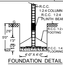
FOUNDATION DETAIL
